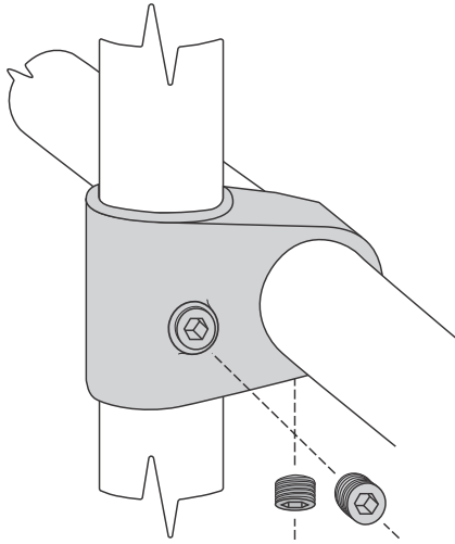
2 x 8mm Allen head bolts per clamp
