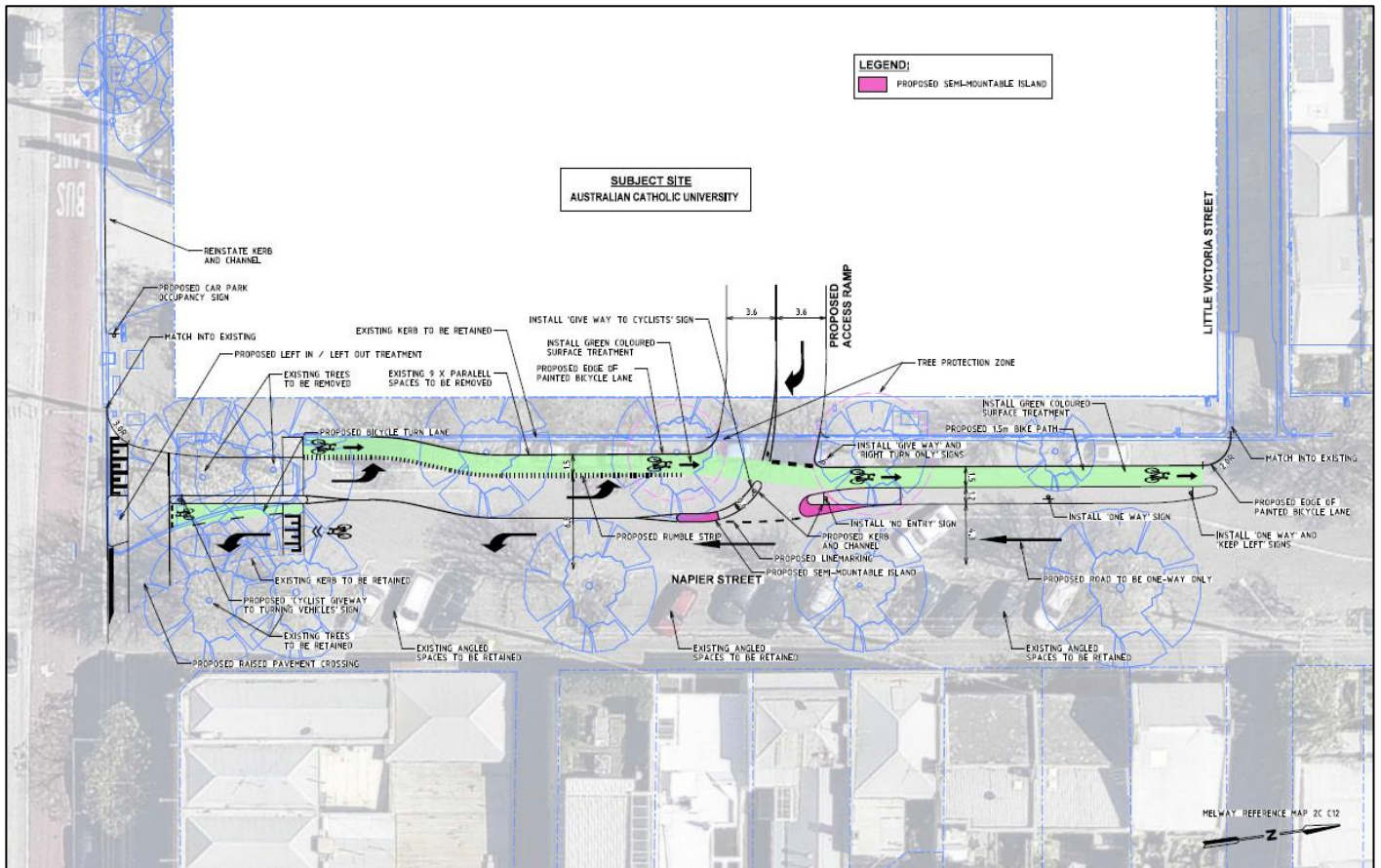
Figure 5-1 Victoria Parade / Napier Street – Concept Design
