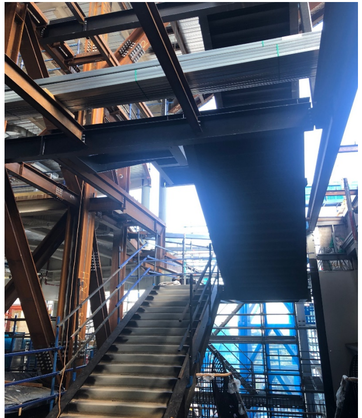
MGB Fish Stair Extension Works
